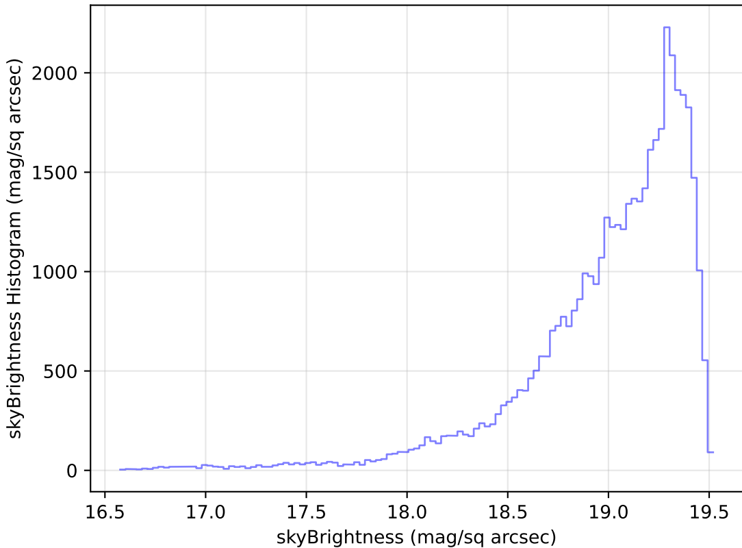
no_magell_roll_v3.4_10yrs Yr 1 z band: skyBrightness Histogram
