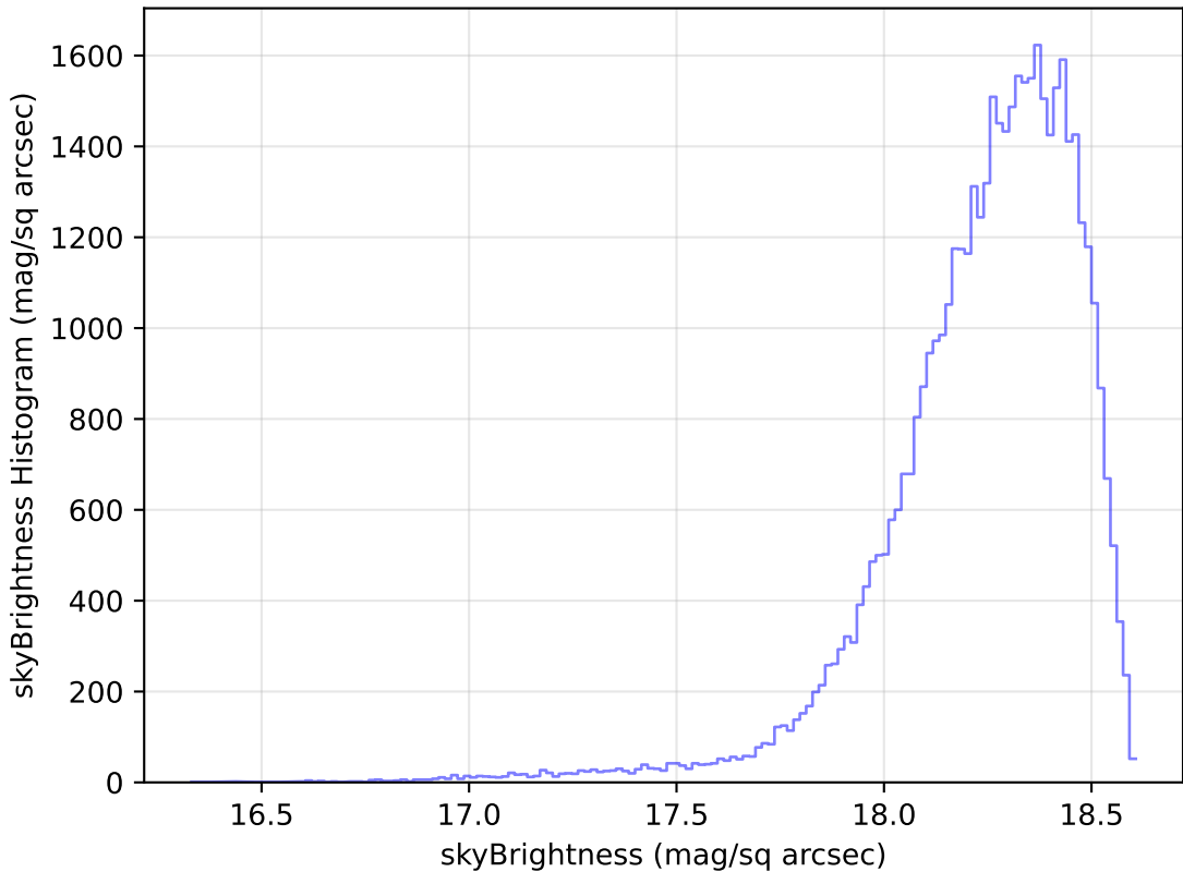
no_magell_roll_v3.4_10yrs Yr 1 y band: skyBrightness Histogram
