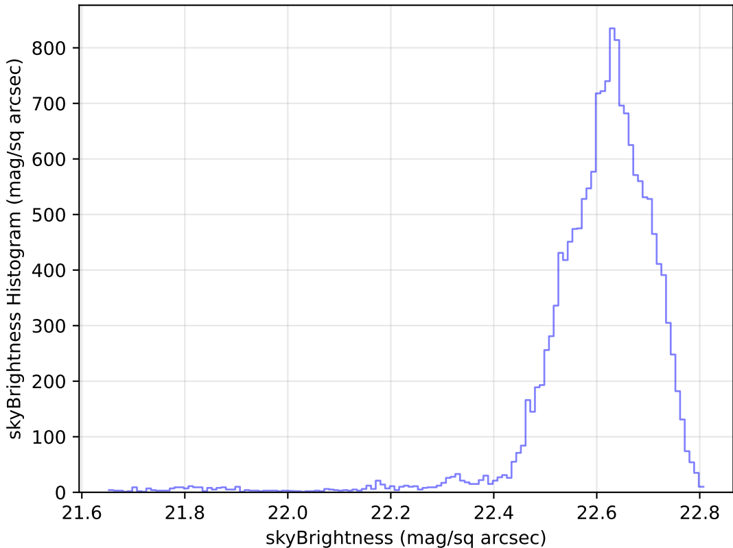
no_magell_roll_v3.4_10yrs Yr 1 u band: skyBrightness Histogram
