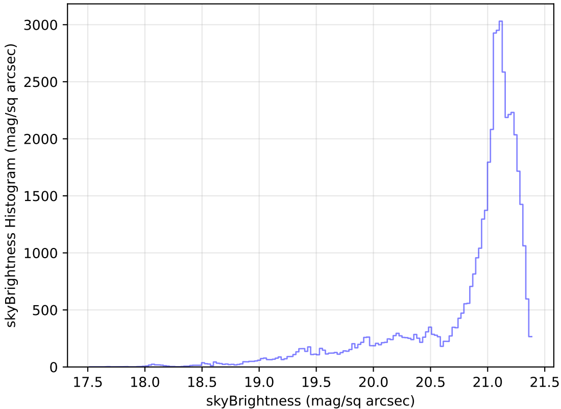
no_magell_roll_v3.4_10yrs Yr 1 r band: skyBrightness Histogram
