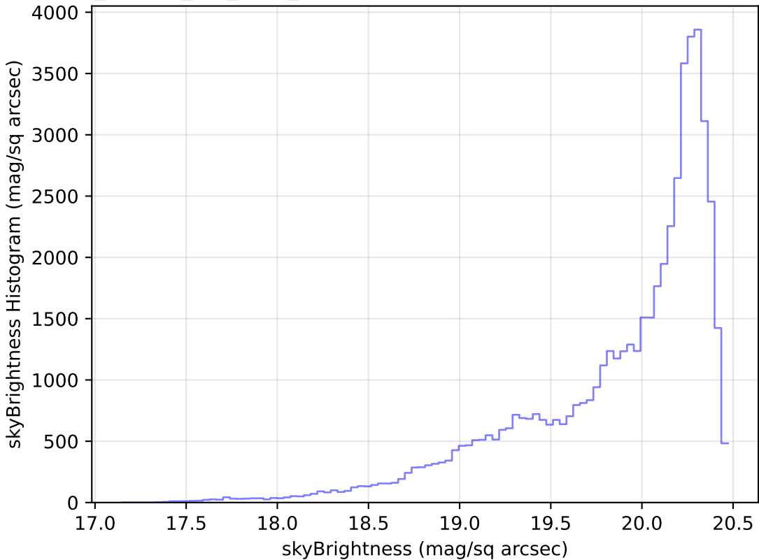
no_magell_roll_v3.4_10yrs Yr 1 i band: skyBrightness Histogram
