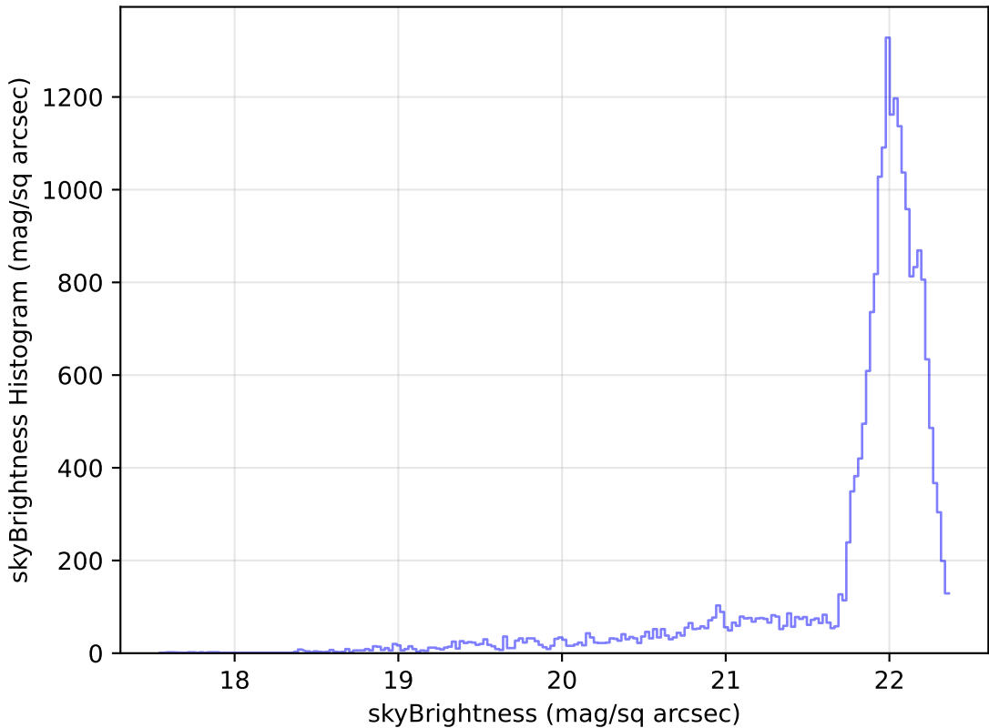
no_magell_roll_v3.4_10yrs Yr 1 g band: skyBrightness Histogram
