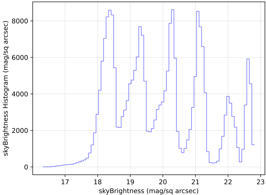
no_magell_roll_v3.4_10yrs Yr 1 all bands: skyBrightness Histogram
