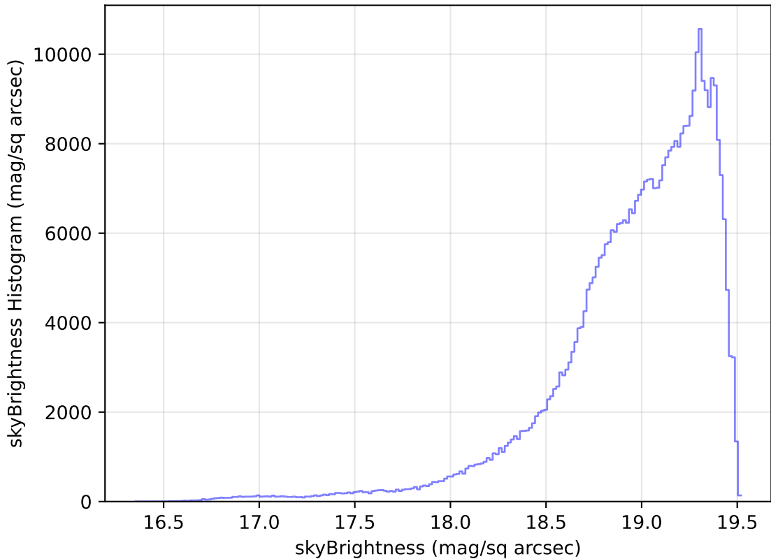
no_magell_roll_v3.4_10yrs WFD z band: skyBrightness Histogram
