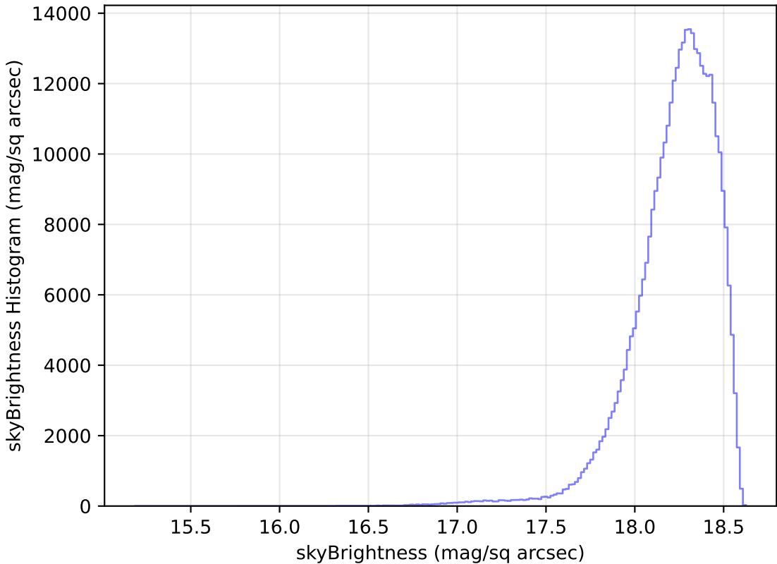
no_magell_roll_v3.4_10yrs WFD y band: skyBrightness Histogram
