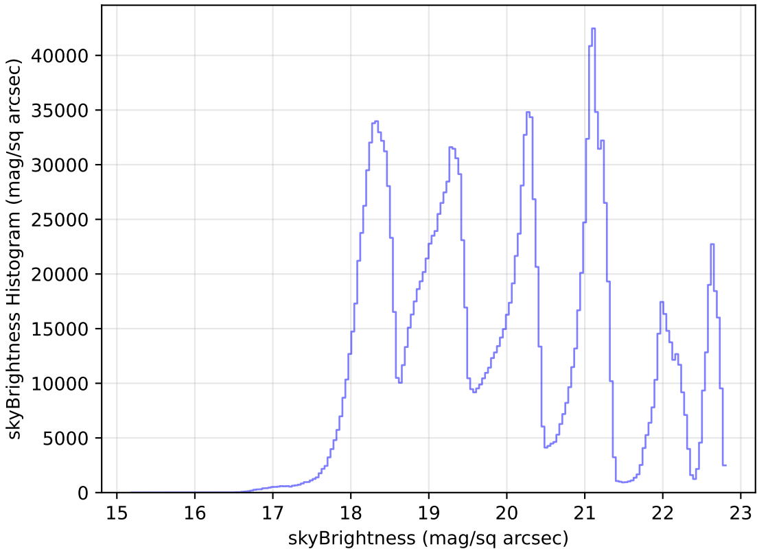
no_magell_roll_v3.4_10yrs WFD all bands: skyBrightness Histogram
