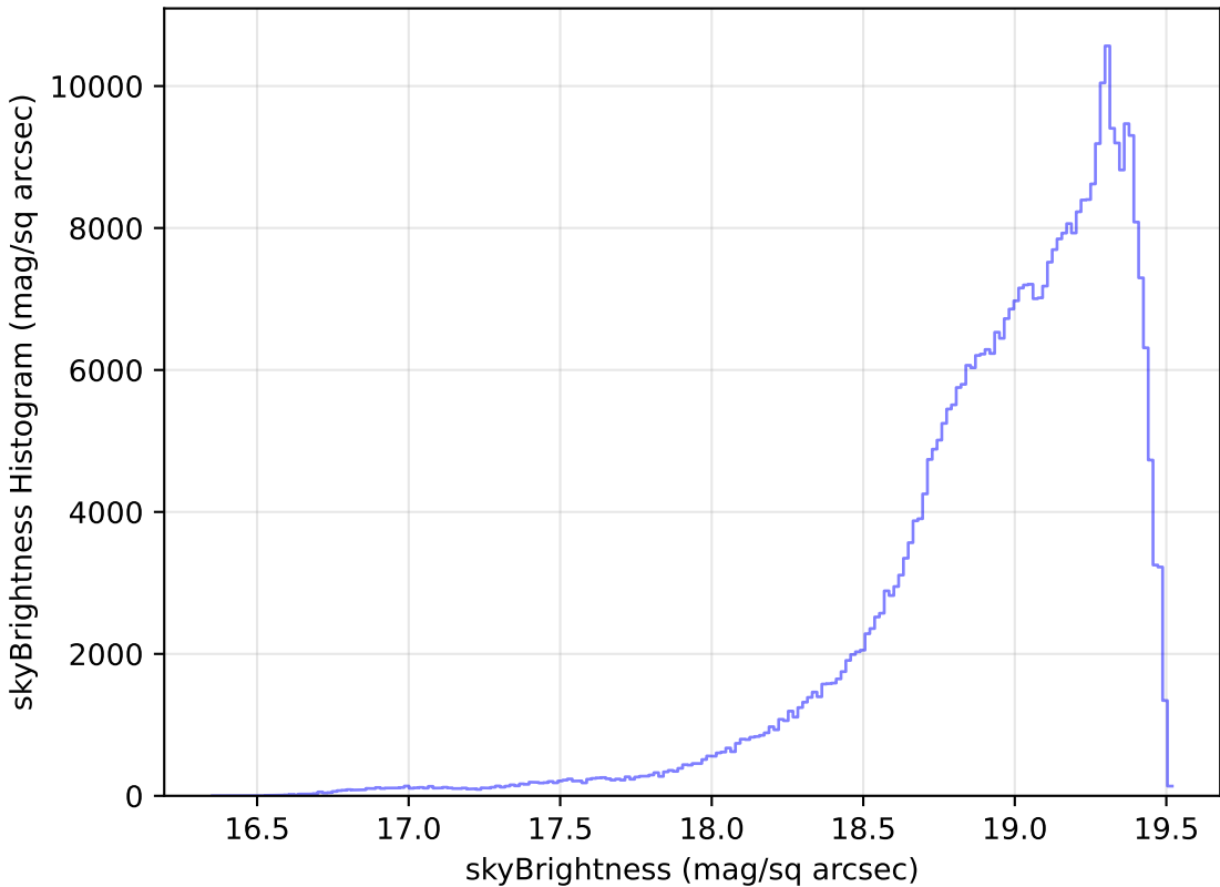
no_magell_roll_v3.4_10yrs All sky z band: skyBrightness Histogram
