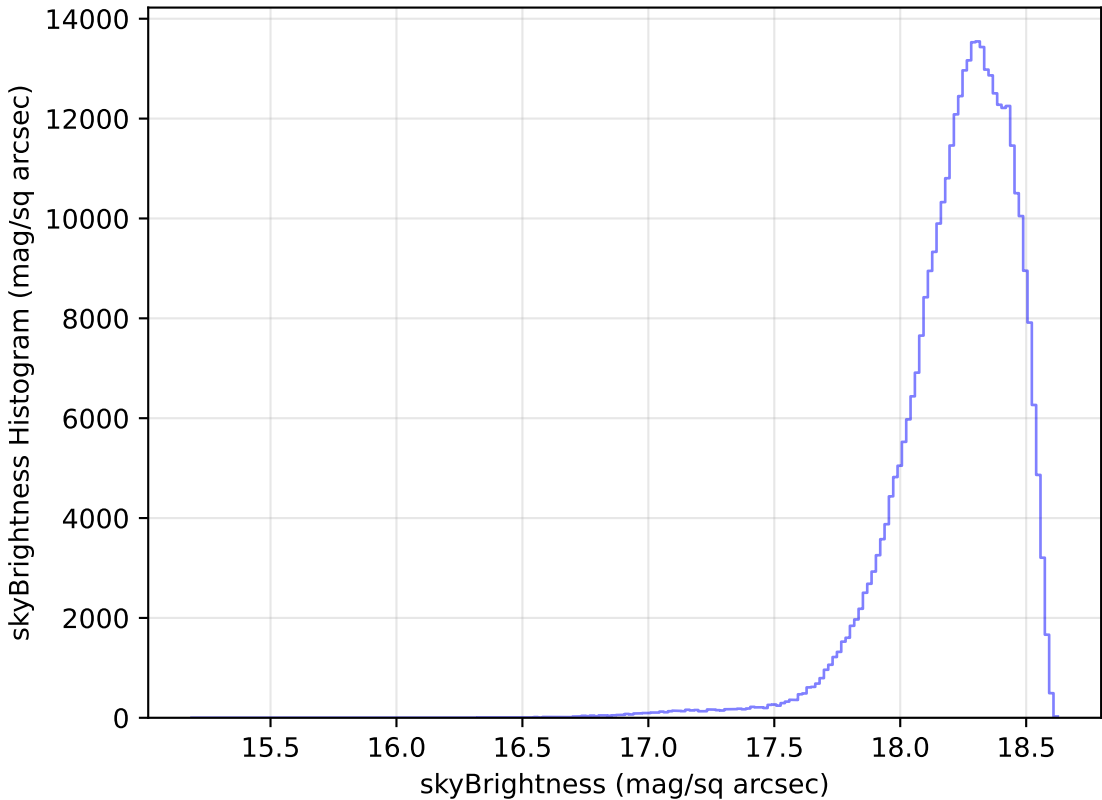
no_magell_roll_v3.4_10yrs All sky y band: skyBrightness Histogram
