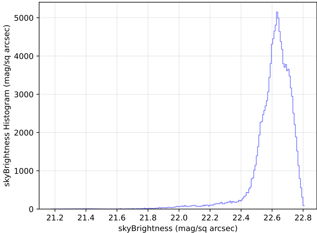
no_magell_roll_v3.4_10yrs All sky u band: skyBrightness Histogram
