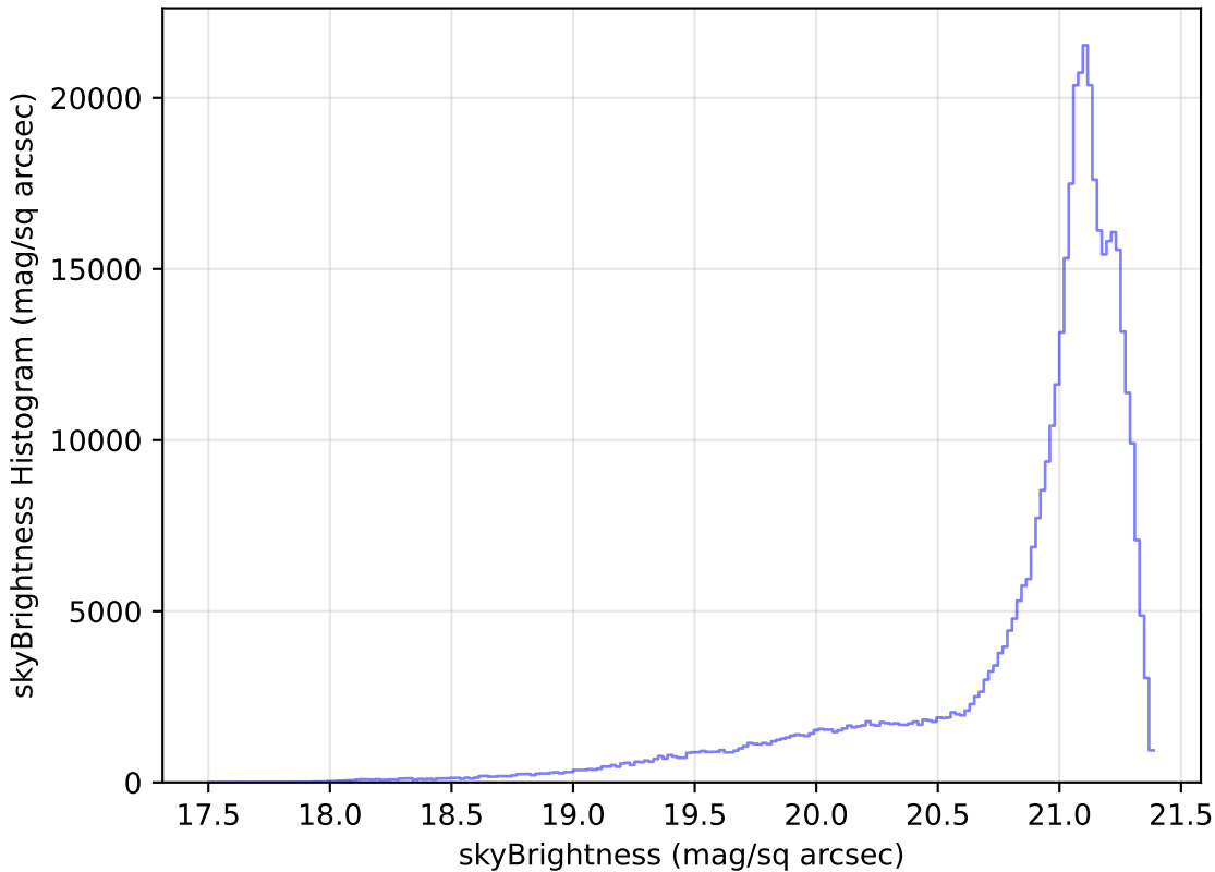
no_magell_roll_v3.4_10yrs All sky r band: skyBrightness Histogram
