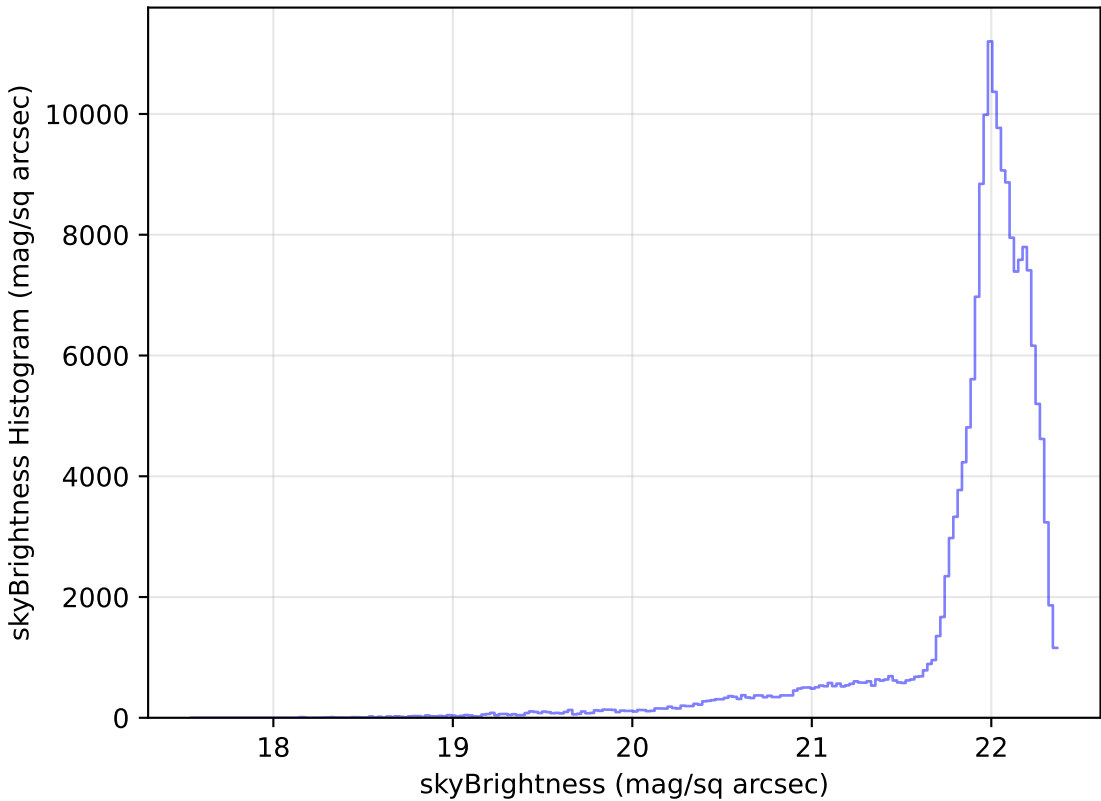
no_magell_roll_v3.4_10yrs All sky g band: skyBrightness Histogram
