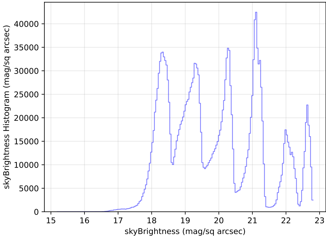
no_magell_roll_v3.4_10yrs All sky all bands: skyBrightness Histogram
