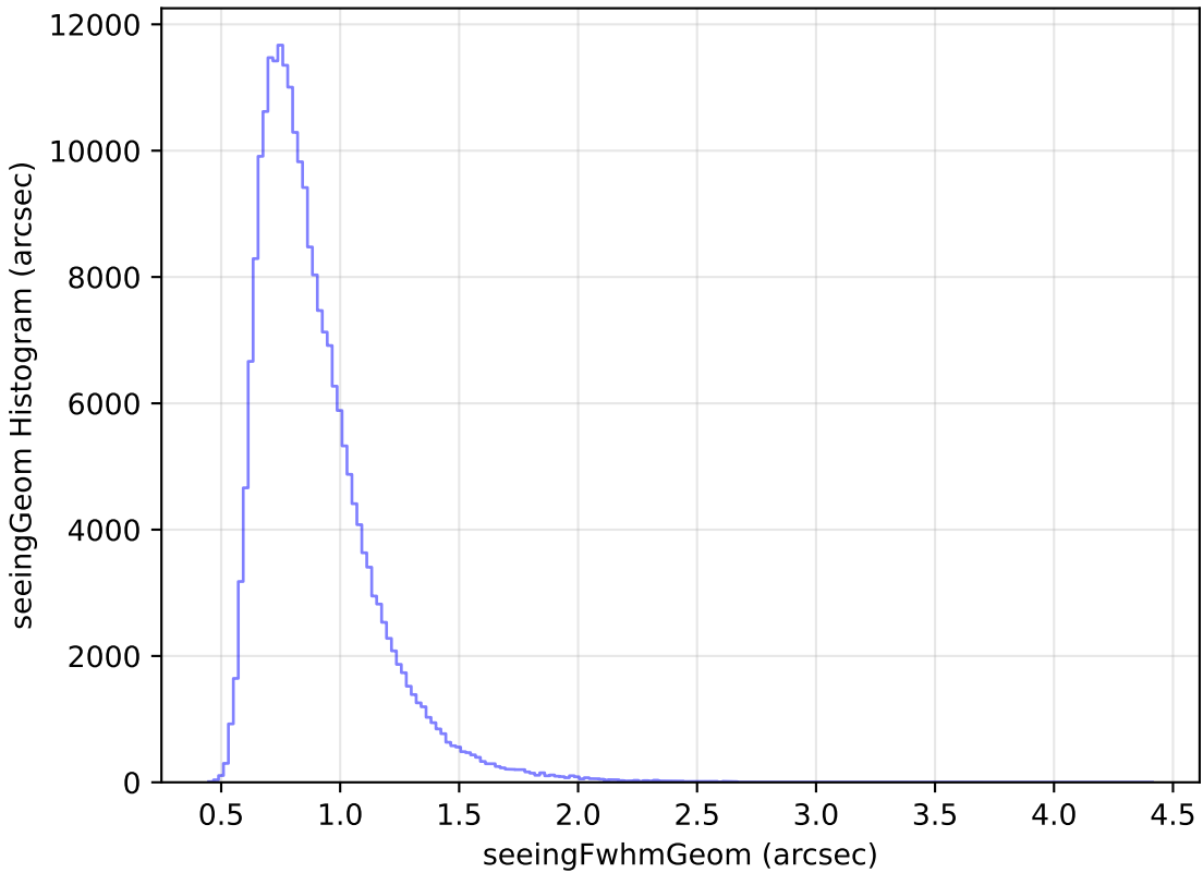
no_magell_roll_v3.4_10yrs Yr 1 all bands: seeingGeom Histogram
