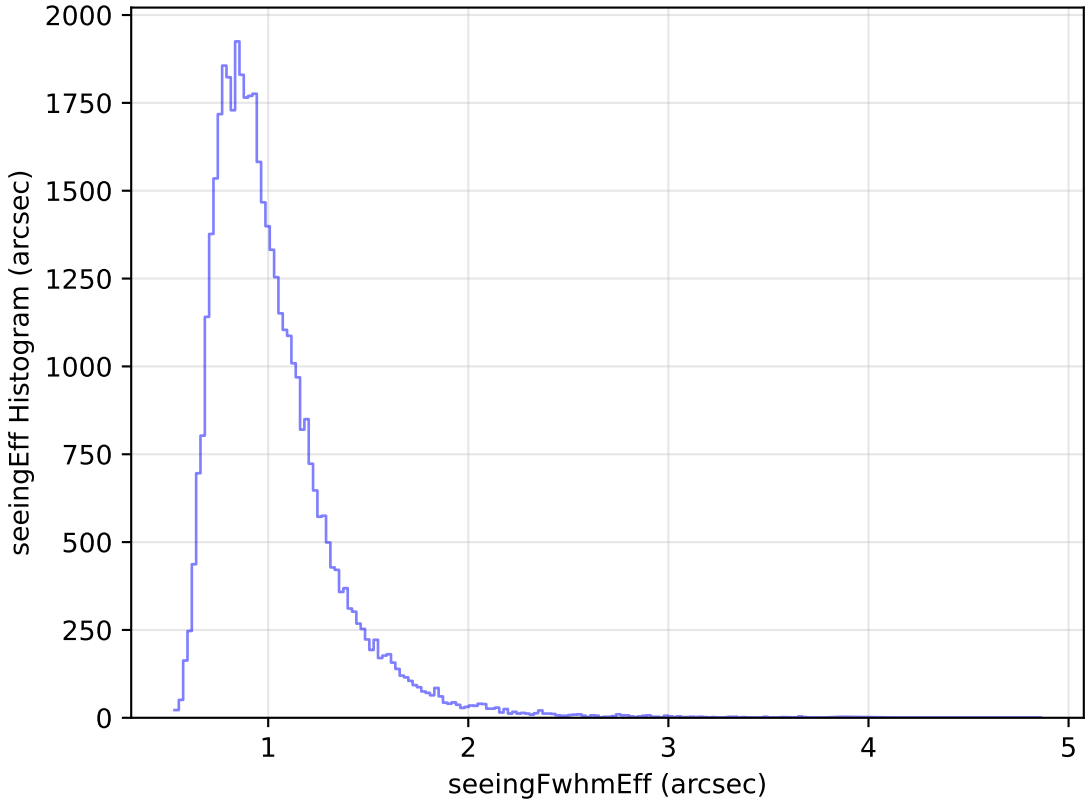
no_magell_roll_v3.4_10yrs Yr 1 z band: seeingEff Histogram
