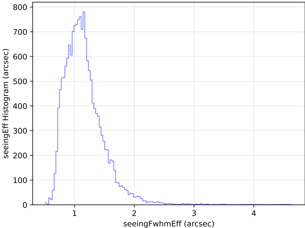
no_magell_roll_v3.4_10yrs Yr 1 u band: seeingEff Histogram
