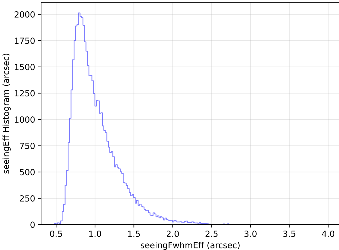
no_magell_roll_v3.4_10yrs Yr 1 r band: seeingEff Histogram
