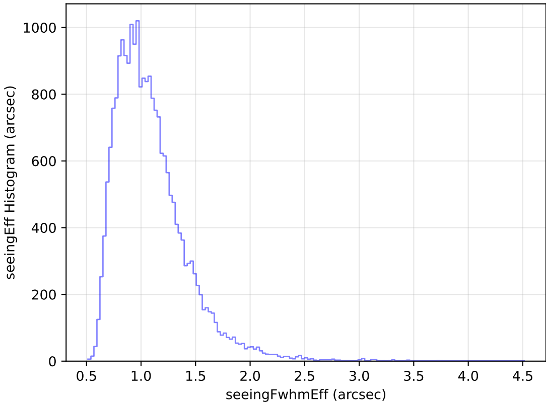
no_magell_roll_v3.4_10yrs Yr 1 g band: seeingEff Histogram
