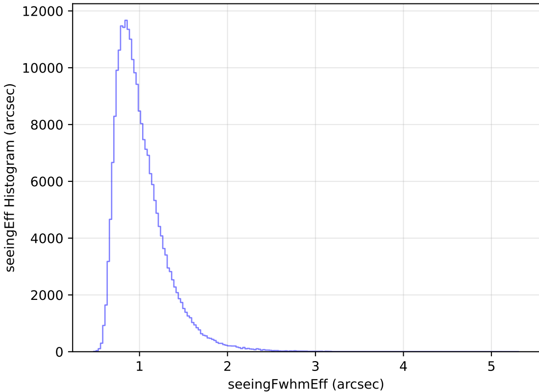
no_magell_roll_v3.4_10yrs Yr 1 all bands: seeingEff Histogram
