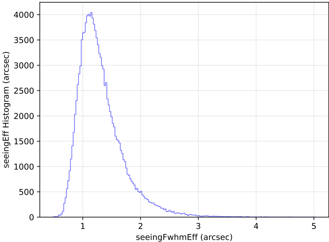
no_magell_roll_v3.4_10yrs WFD u band: seeingEff Histogram
