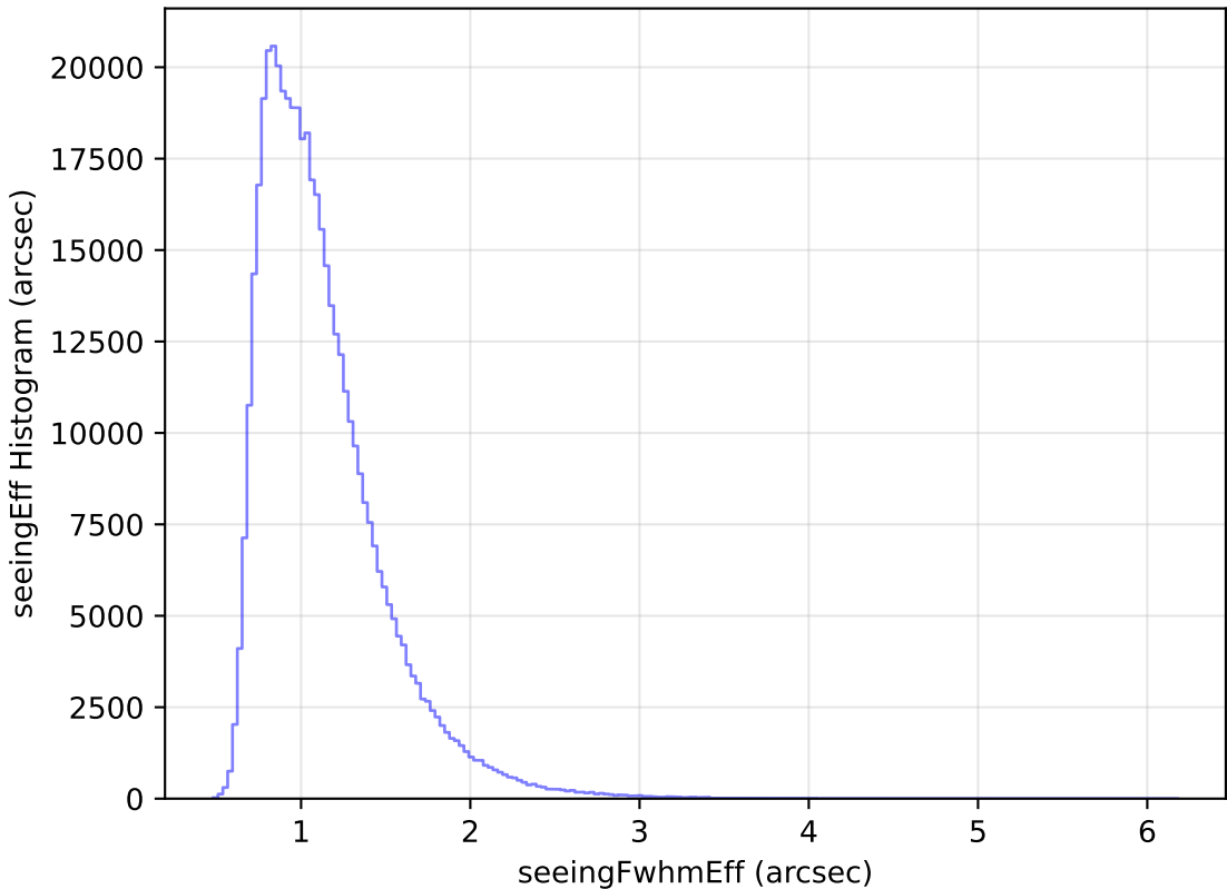
no_magell_roll_v3.4_10yrs WFD r band: seeingEff Histogram
