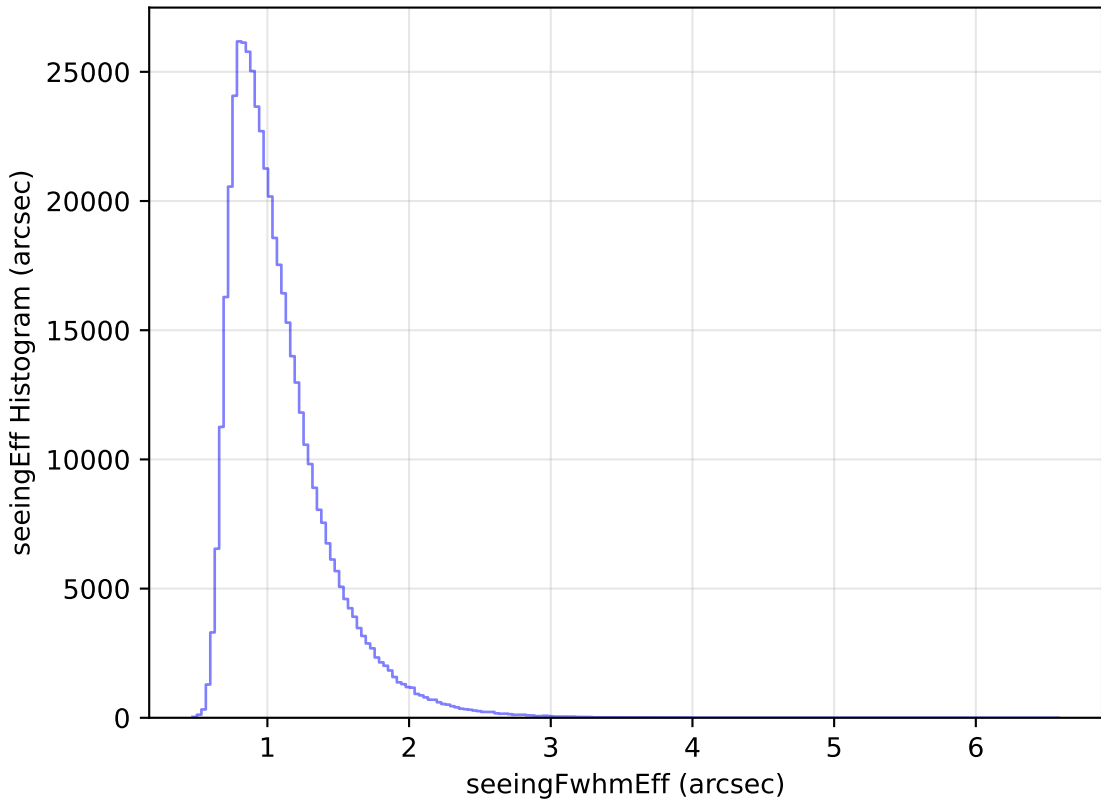
no_magell_roll_v3.4_10yrs WFD i band: seeingEff Histogram
