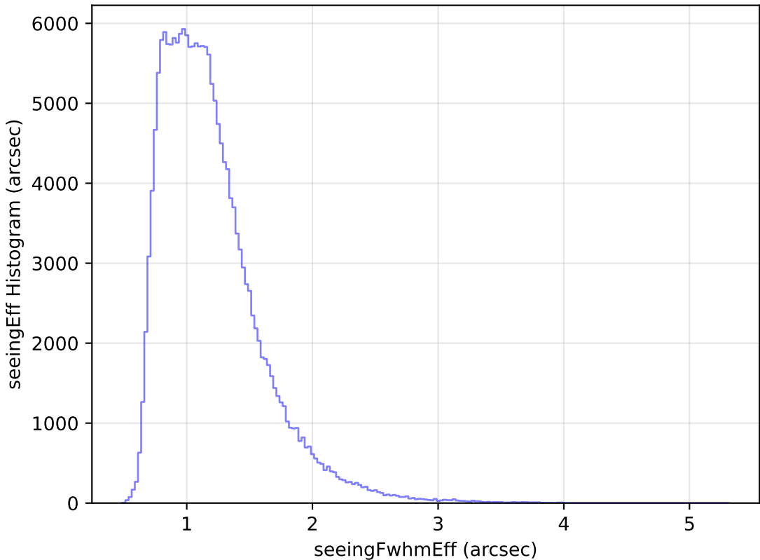
no_magell_roll_v3.4_10yrs WFD g band: seeingEff Histogram
