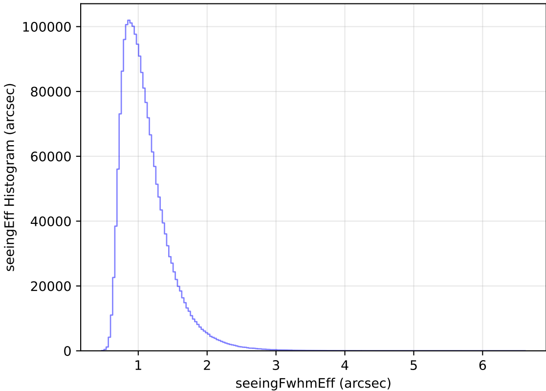
no_magell_roll_v3.4_10yrs WFD all bands: seeingEff Histogram
