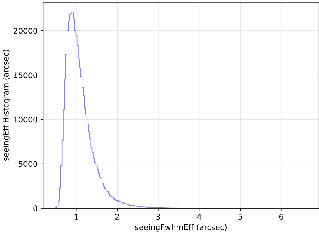
no_magell_roll_v3.4_10yrs All sky z band: seeingEff Histogram
