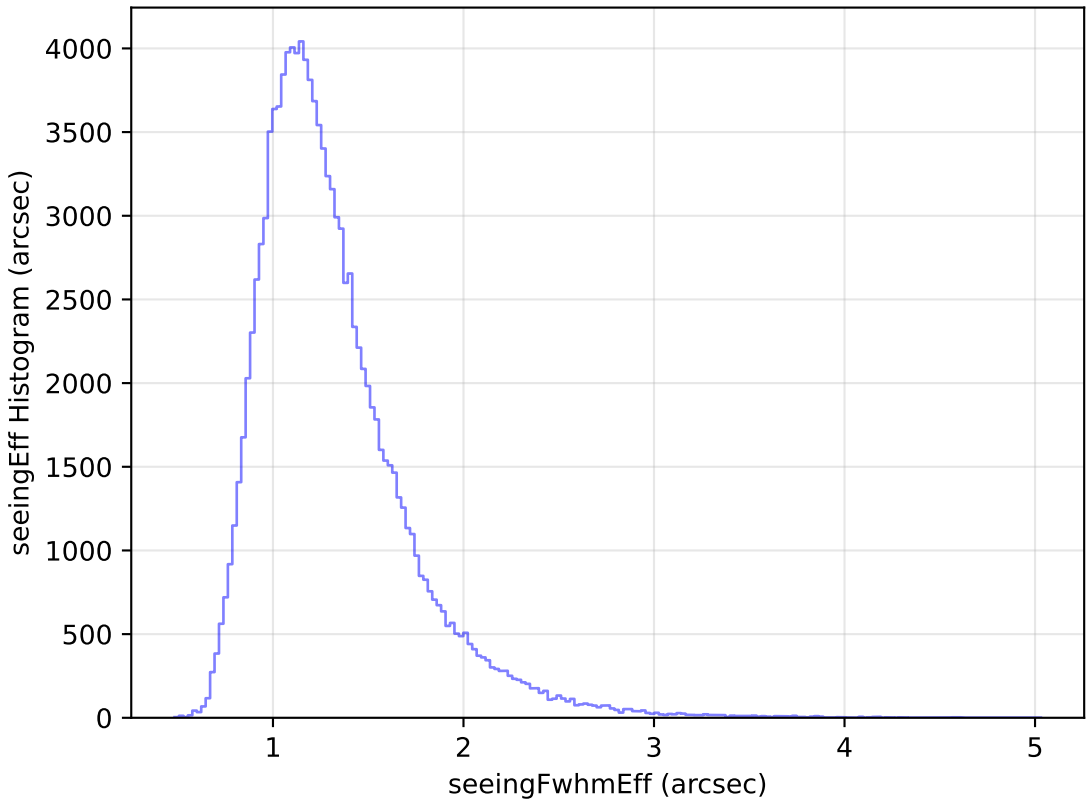
no_magell_roll_v3.4_10yrs All sky u band: seeingEff Histogram
