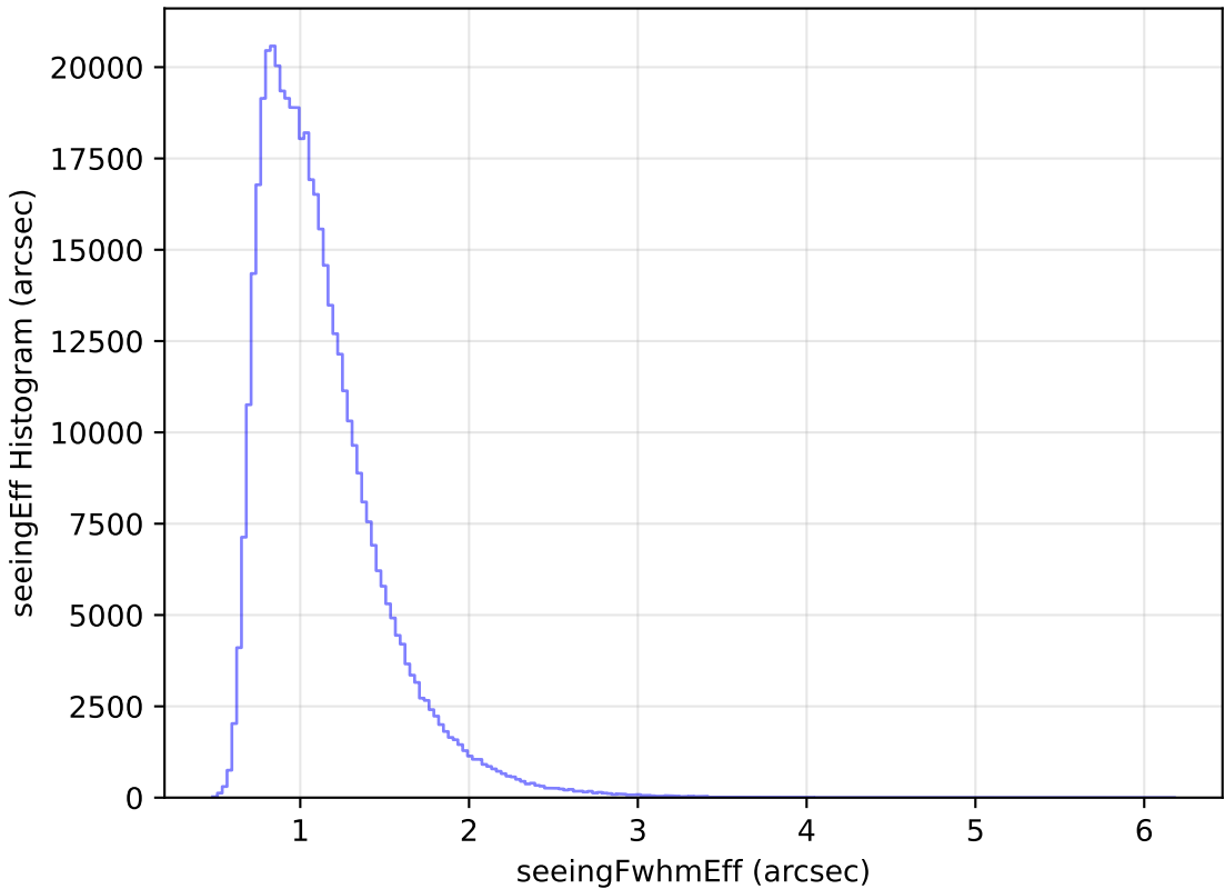
no_magell_roll_v3.4_10yrs All sky r band: seeingEff Histogram
