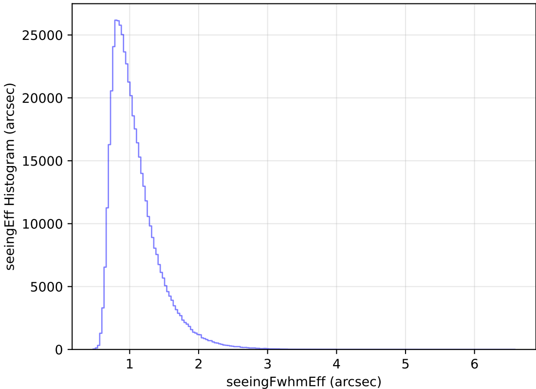
no_magell_roll_v3.4_10yrs All sky i band: seeingEff Histogram
