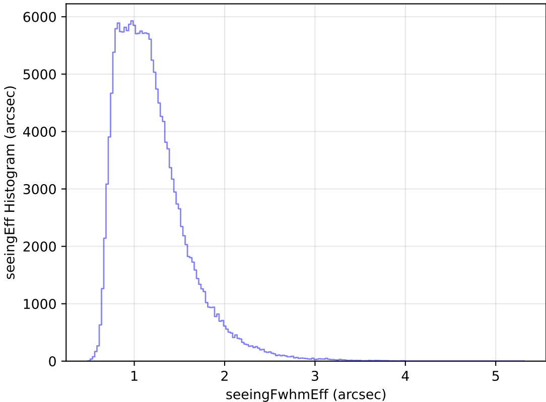
no_magell_roll_v3.4_10yrs All sky g band: seeingEff Histogram
