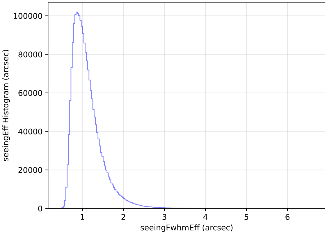
no_magell_roll_v3.4_10yrs All sky all bands: seeingEff Histogram
