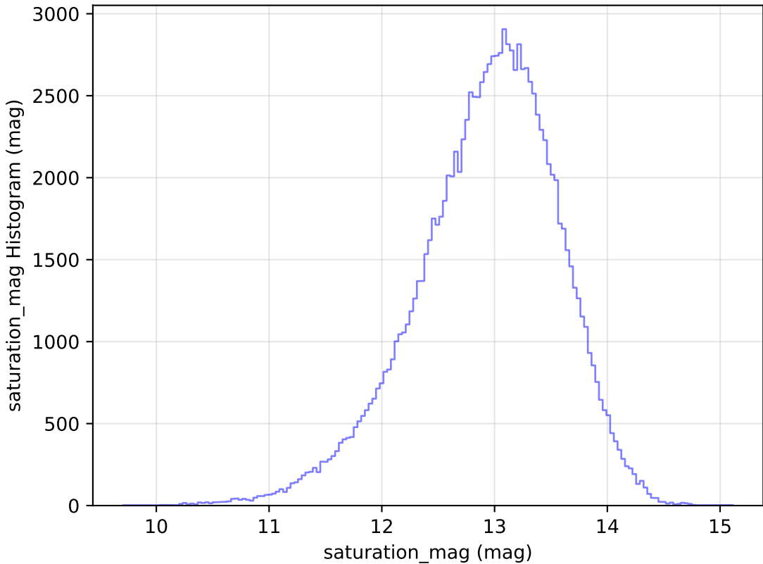
no_magell_roll_v3.4_10yrs WFD u band: saturation_mag Histogram
