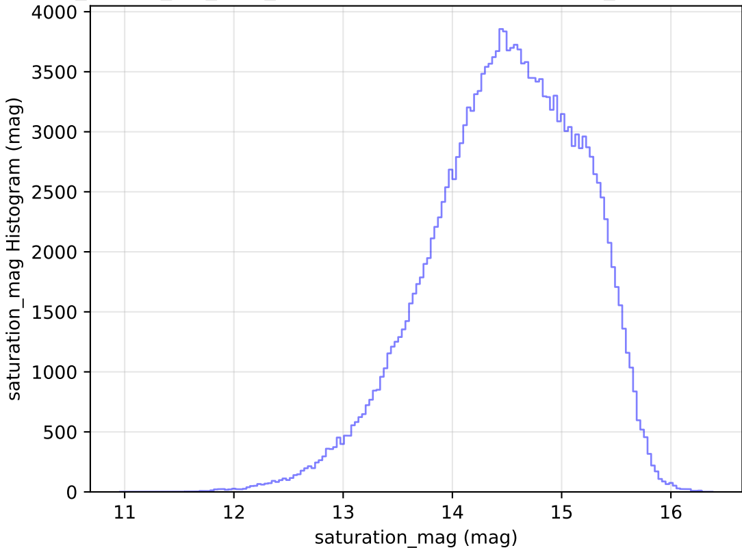
no_magell_roll_v3.4_10yrs WFD g band: saturation_mag Histogram
