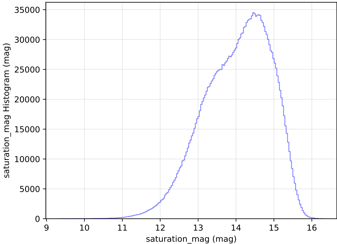
no_magell_roll_v3.4_10yrs WFD all bands: saturation_mag Histogram
