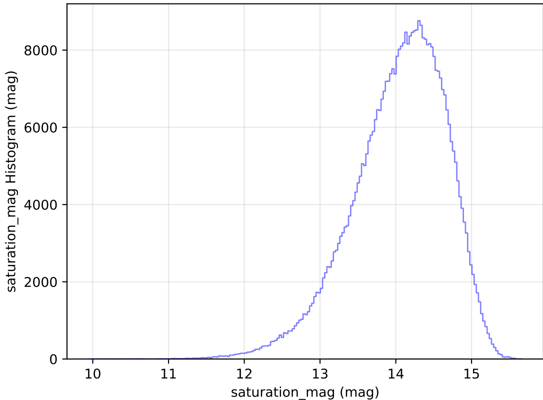
no_magell_roll_v3.4_10yrs All sky z band: saturation_mag Histogram
