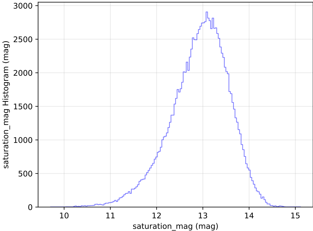
no_magell_roll_v3.4_10yrs All sky u band: saturation_mag Histogram
