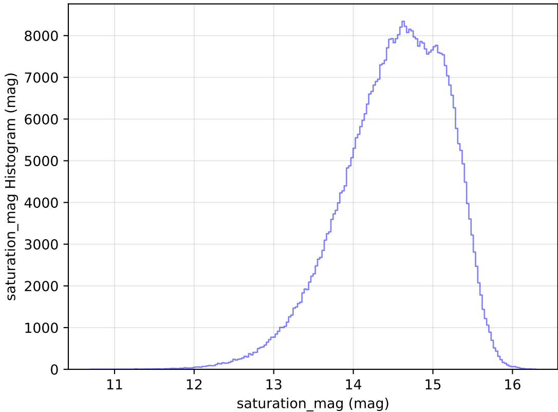
no_magell_roll_v3.4_10yrs All sky r band: saturation_mag Histogram
