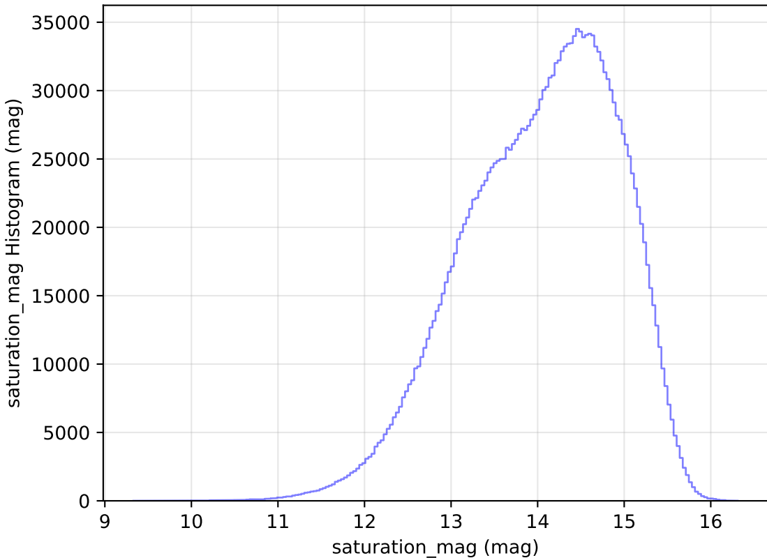
no_magell_roll_v3.4_10yrs All sky all bands: saturation_mag Histogram
