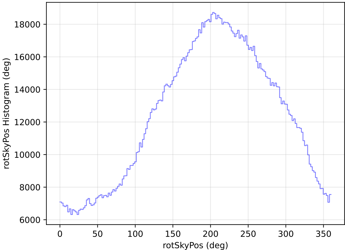
no_magell_roll_v3.4_10yrs WFD all bands: rotSkyPos Histogram
