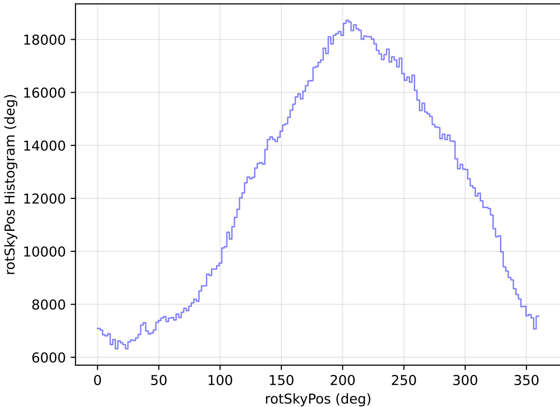
no_magell_roll_v3.4_10yrs All sky all bands: rotSkyPos Histogram
