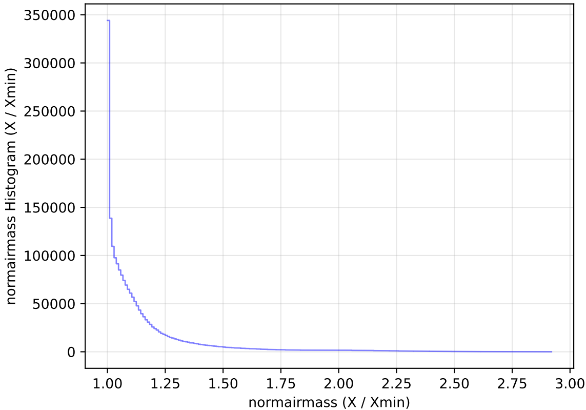
no_magell_roll_v3.4_10yrs All sky all bands: normairmass Histogram
