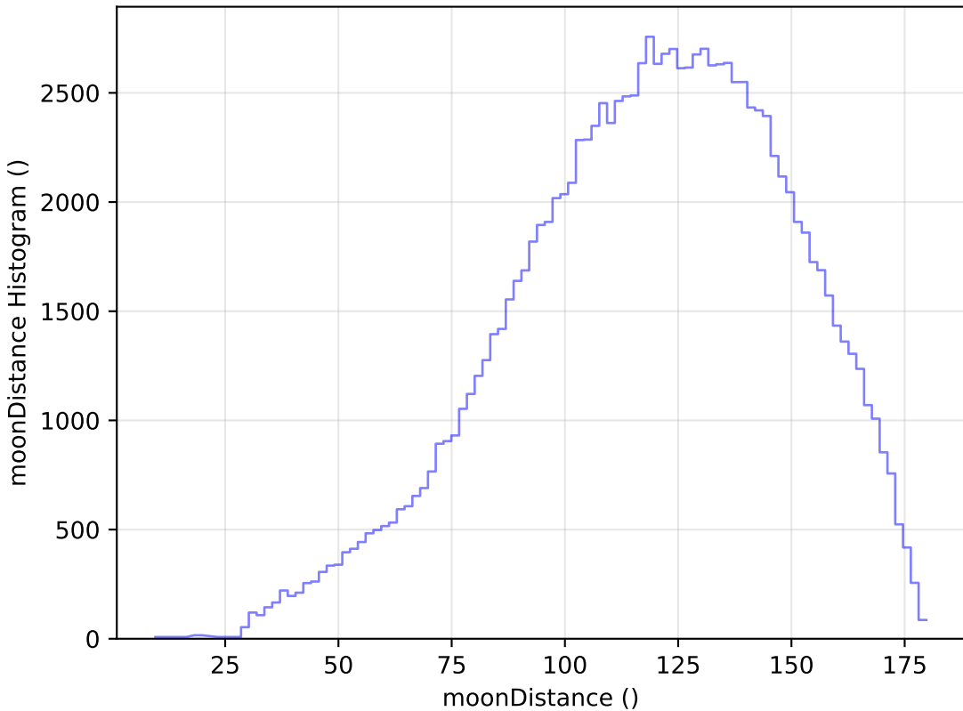
no_magell_roll_v3.4_10yrs WFD u band: moonDistance Histogram
