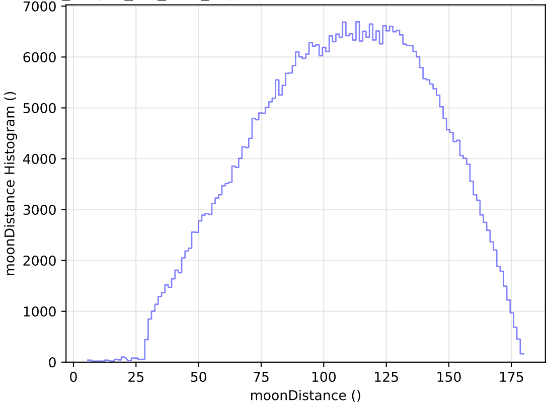
no_magell_roll_v3.4_10yrs WFD r band: moonDistance Histogram
