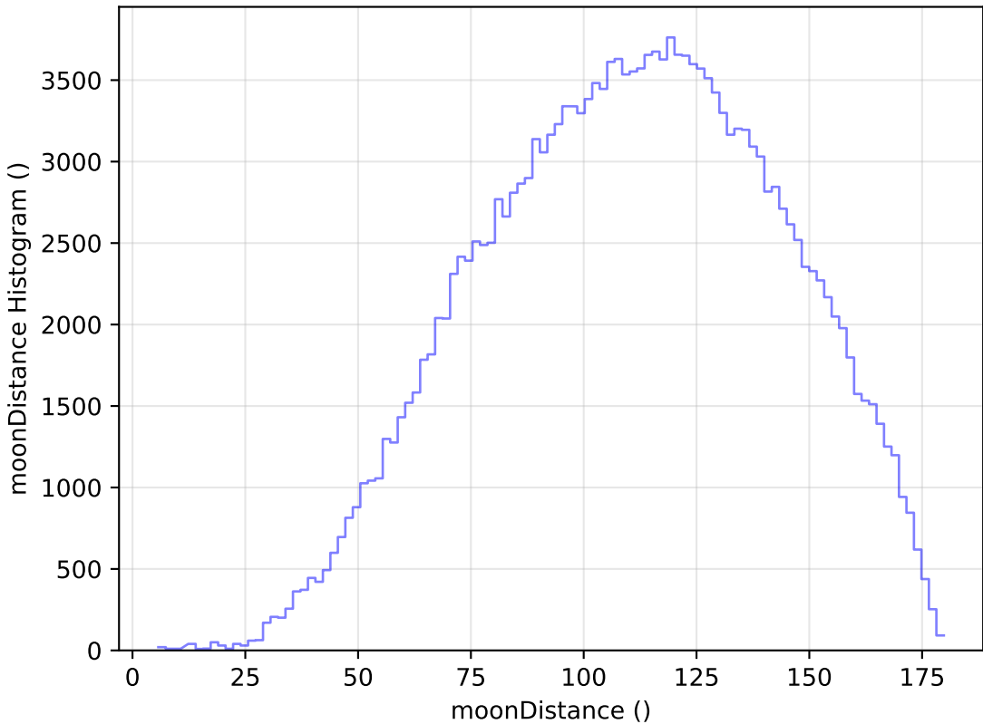
no_magell_roll_v3.4_10yrs WFD g band: moonDistance Histogram
