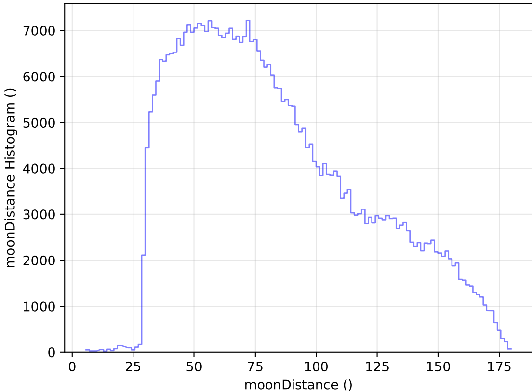
no_magell_roll_v3.4_10yrs All sky z band: moonDistance Histogram
