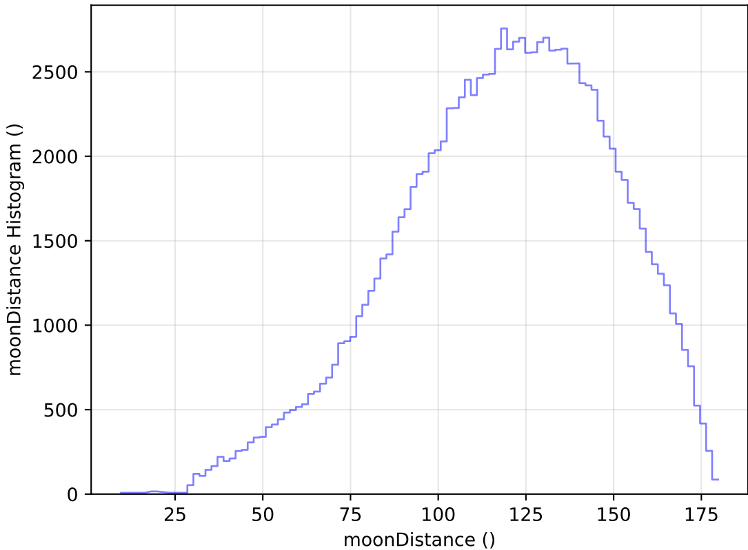
no_magell_roll_v3.4_10yrs All sky u band: moonDistance Histogram
