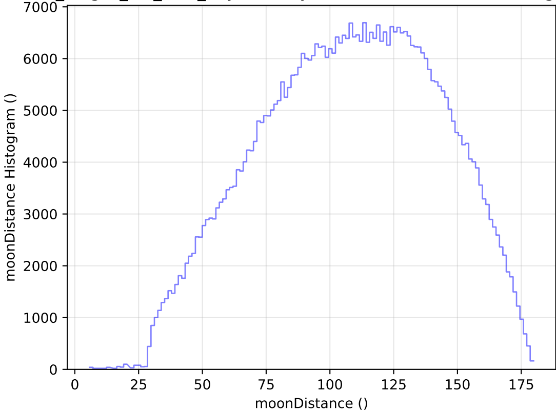
no_magell_roll_v3.4_10yrs All sky r band: moonDistance Histogram
