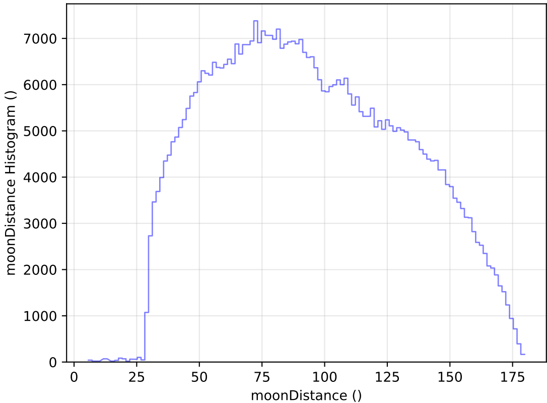
no_magell_roll_v3.4_10yrs All sky i band: moonDistance Histogram
